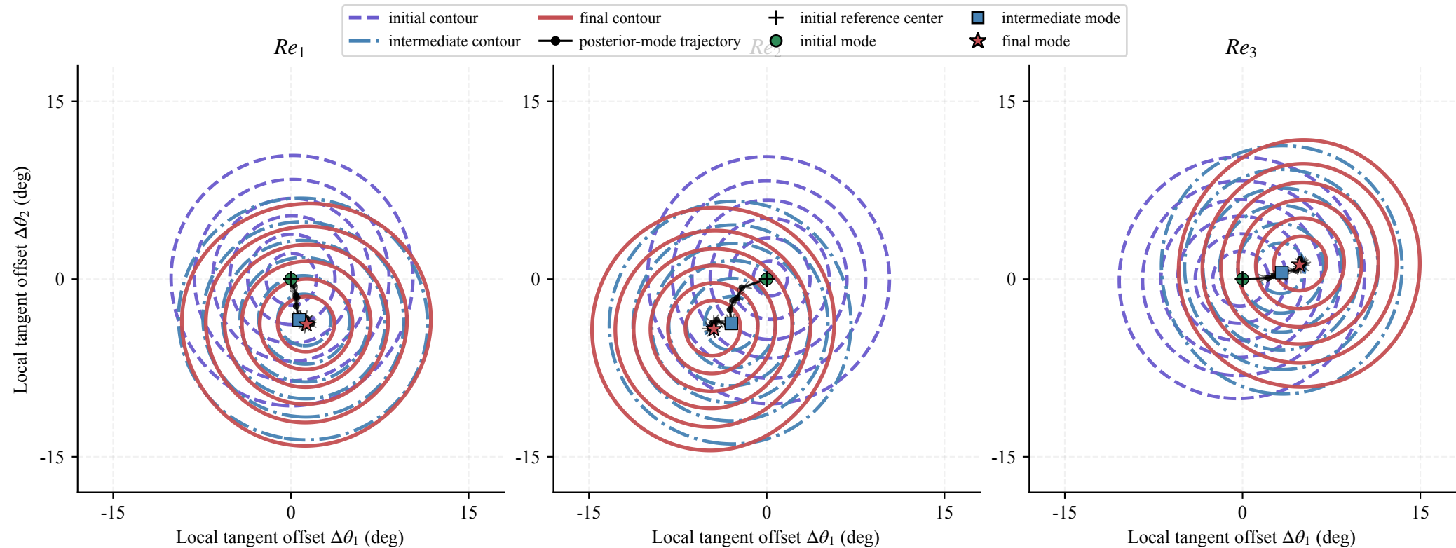
Local contour evolution and posterior-mode migration of rotational marginals
